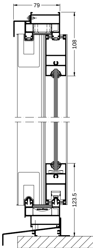
Vertical section detail of Schüco TropTec AS 39 SC.NI Scale 1:4 Vertikalschnitt Schüco TropTec AS 39 SC.NI Maßstab 1:4
