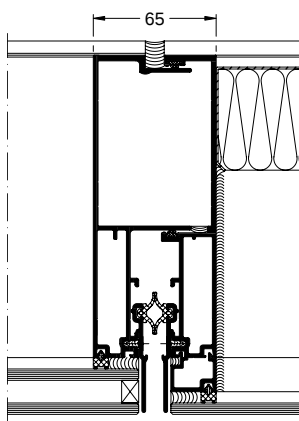
Horizontal section detail of Schüco TropTec UC 65 SG.NI Scale 1:4
